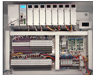
PLC Hydraulic System Control
